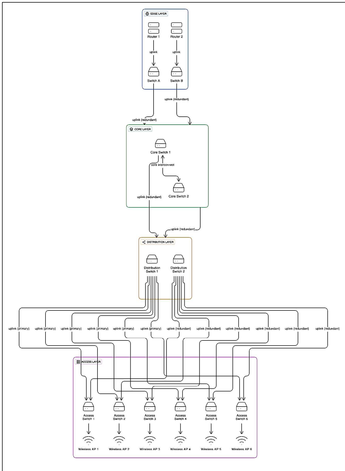
Figure E.4.1 - Typical IT Network Topology
