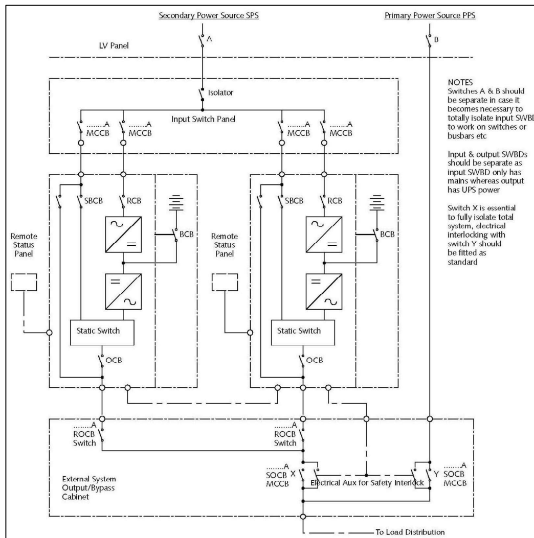
Figure: Synchronous / Parallel Redundant UPS Arrangement
